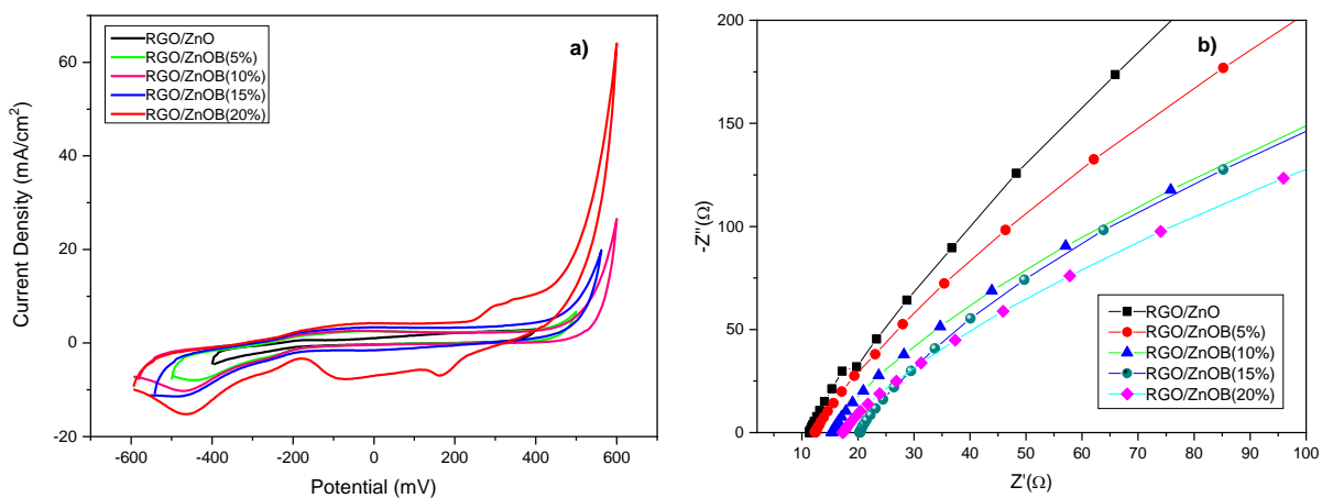
Fig. 4. (a) The cyclic voltammogram graphic and (b) Nyquist impedance spectrum of the Graphite/PTFE/RGO/ZnO:B electrodes under a 5 mV/s scanning rate
