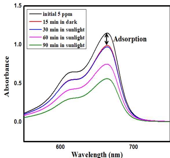
Fig. 12. UV-Visible spectra for degradation of MB under sunlight with CuO films.
