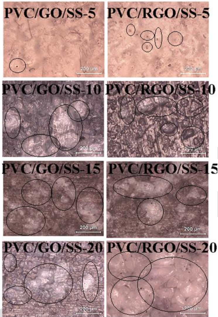
Fig. 7. OM images of hybrid biocomposites at same magnification (10X).
