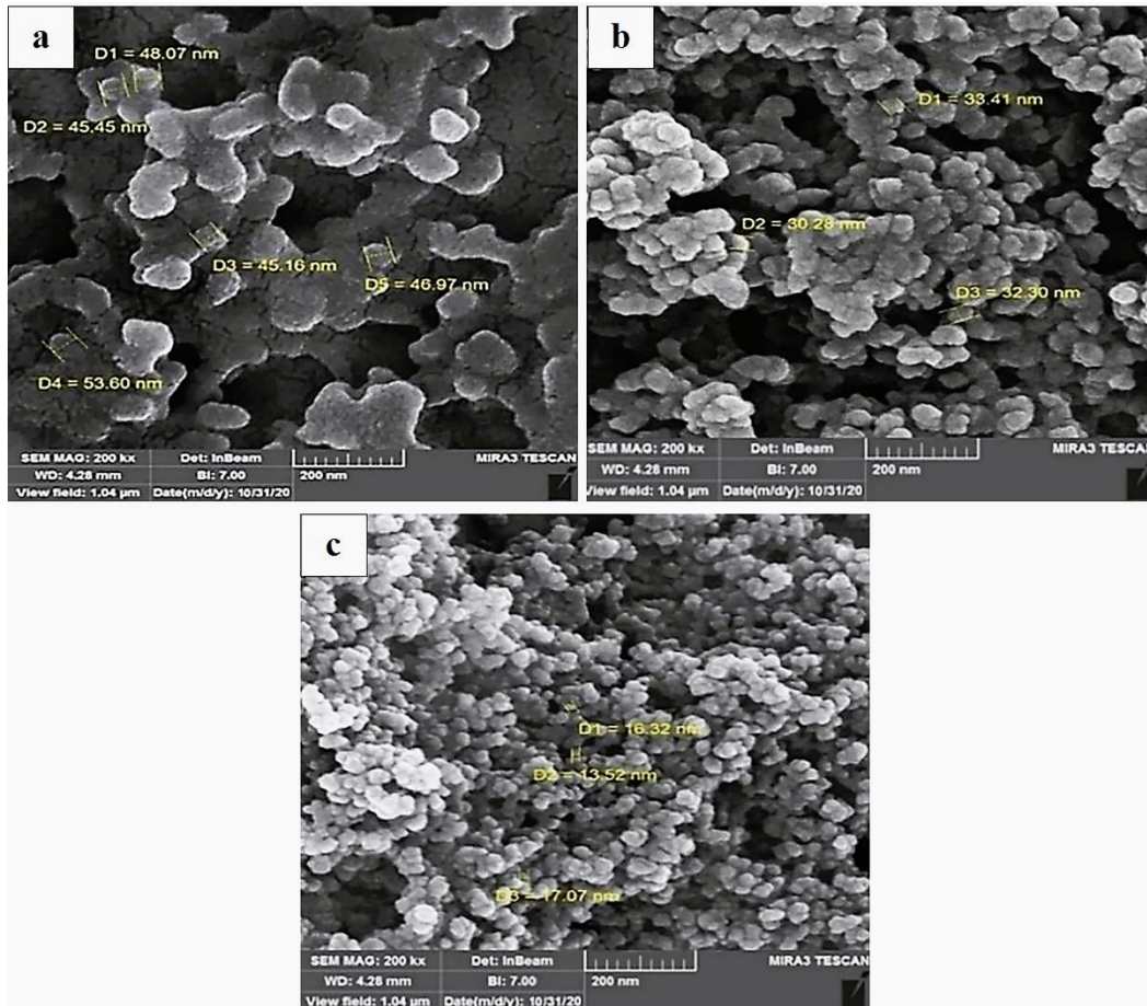
Fig. 3. SEM images of the coatings obtained at a frequency of 10 Hz, duty cycle of 10 % and current density of: a) 0.1, b) 0.2 and c) 0.3 A/cm 2 .
