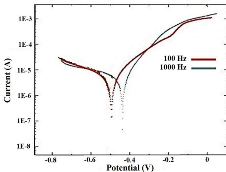
Fig. 9. Tafel curves of the coatings prepared at a current density of 0.2 \text{ A/cm}^2 , duty cycle of 10 % and with varying frequency in a 3.5% NaCl aqueous solution.
