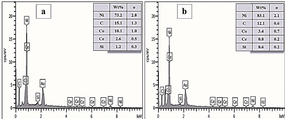
Fig. 4. EDS results of the coatings obtained at a frequency of 10 Hz, duty cycle of 10 % and different current density: a) 0.1, and b) 0.3 \text{A}/\text{cm}^2
