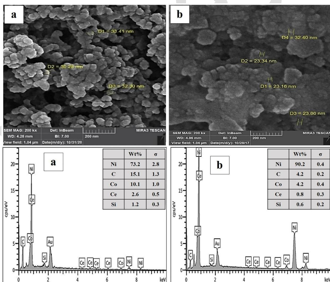
Fig. 6. SEM images and EDS results of the coatings obtained at a current density of 0.2 \text{ A/cm}^2 , a frequency of 10 Hz, and duty cycles: a) 10 %, and b) 30 %.
