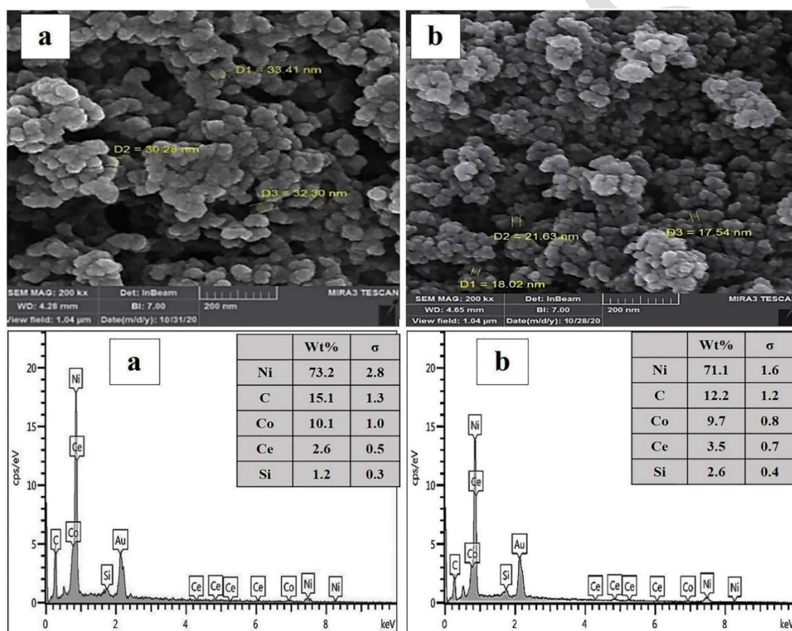
Fig. 8. SEM images and EDS results of the coatings prepared at a current density of 0.2 A/cm 2 , duty cycle of 10 % and with varying frequency: a) 10 Hz, and b) 1000 Hz.
