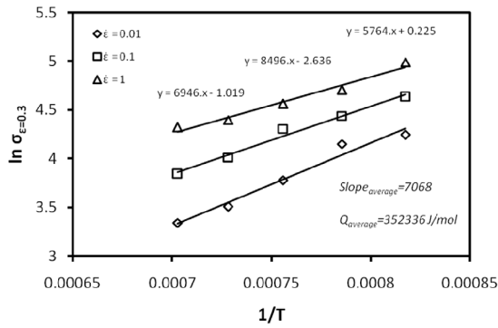
Fig. 3. Diagrams of \ln\sigma_{E=0.3} - 1/T plotted to calculate the average value of Q
