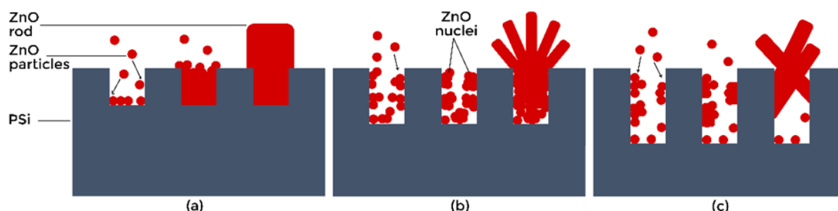
Fig. 3. ZnO rods growth mechanism on the different PSi pore depths: (a) Sample 1 (55 \mu\text{m} ); (b) Sample 2 (180 \mu\text{m} ); (c) Sample 3 (200 \mu\text{m} )
