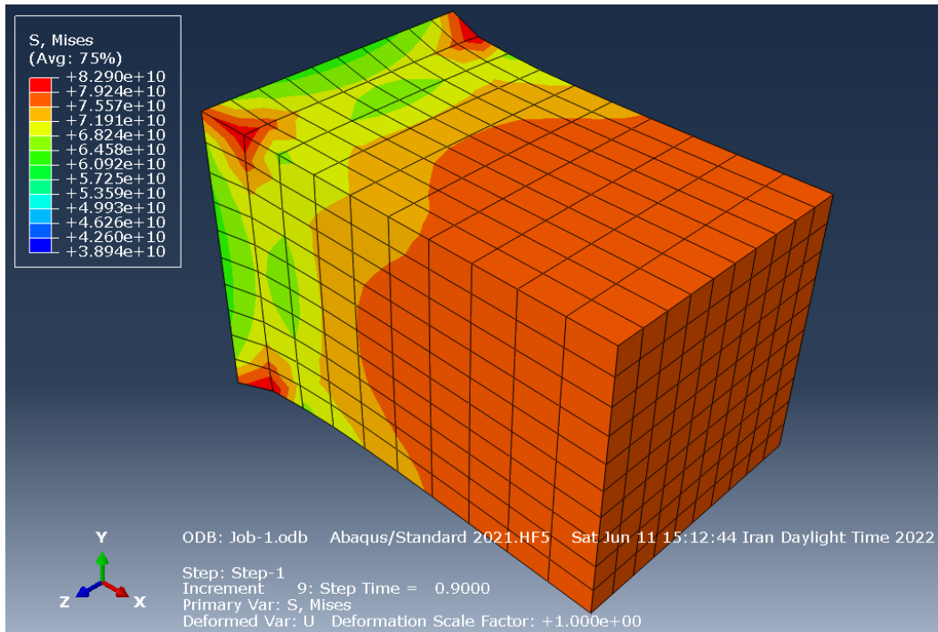
Figure 15. The von-mises stress field of the ABAQUS.
