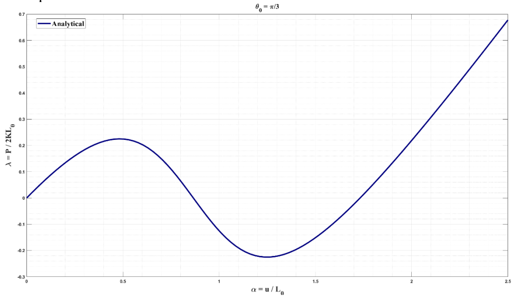
Figure 8. The exact force-displacement curve of example 1.
