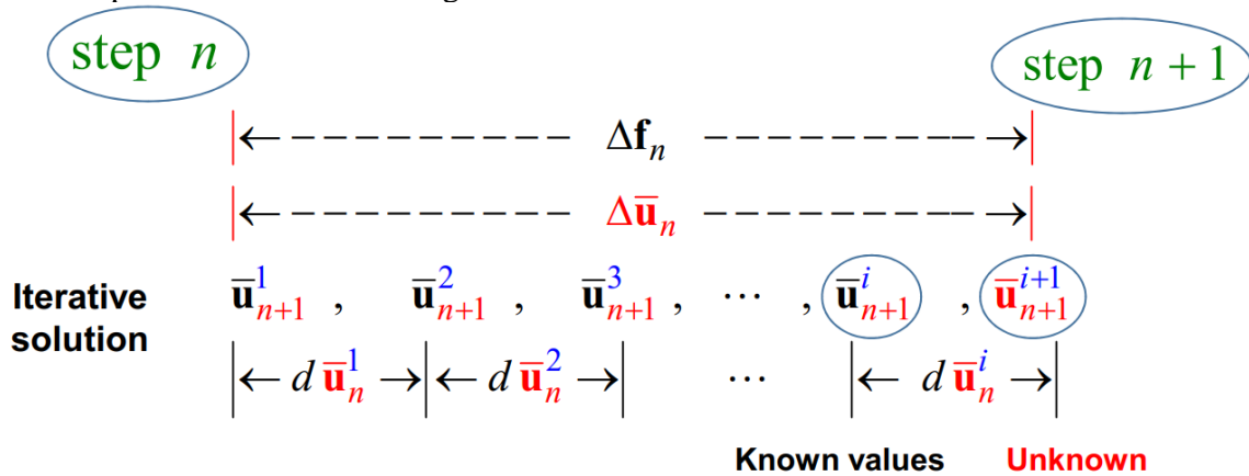
Figure 4. Iterative procedure to obtain unknown variables between steps n and n+1.
