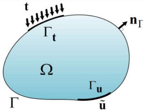
Figure 1. A continuum body in equilibrium.
