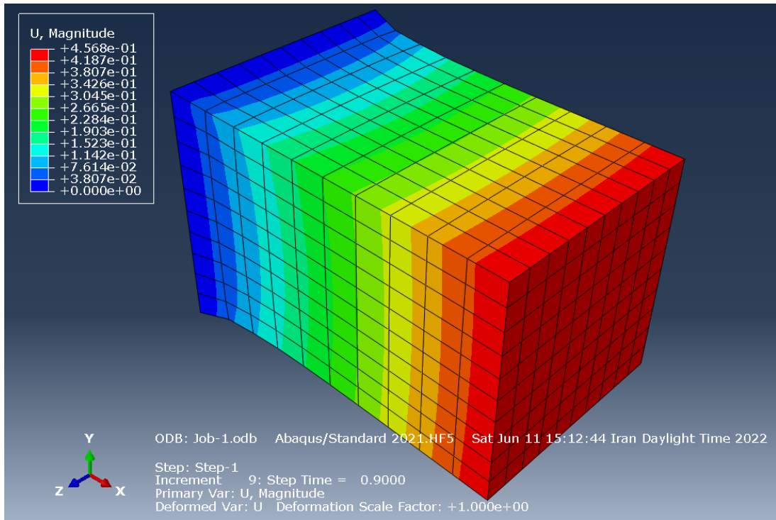
Figure 13. The magnitude displacement field of the ABAQUS.
