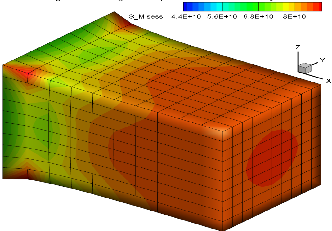
Figure 14. The von-mises stress field of the proposed framework.
