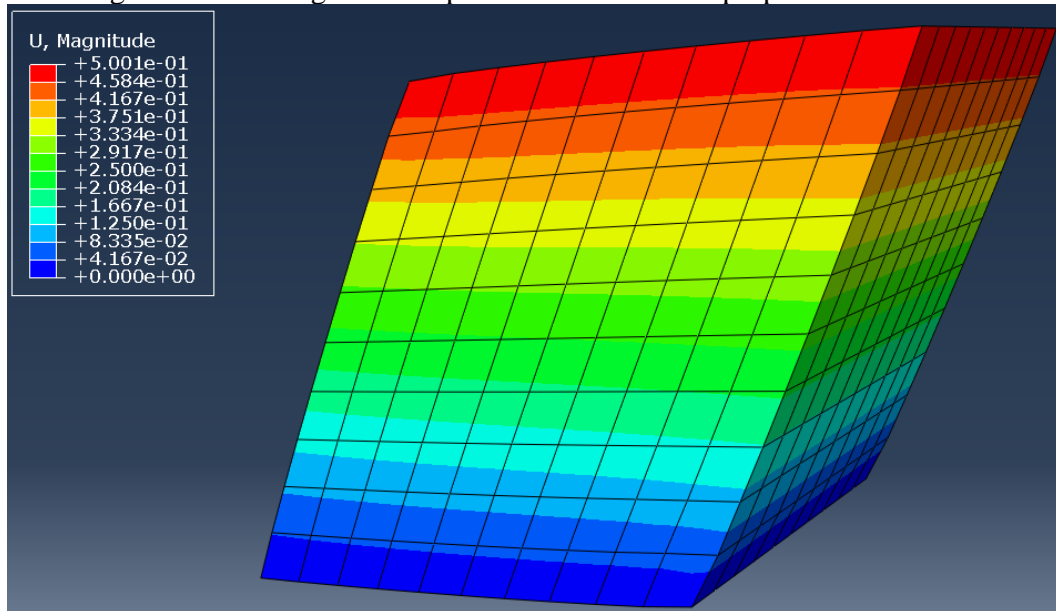
Figure 17. The magnitude displacement field of the ABAQUS.
