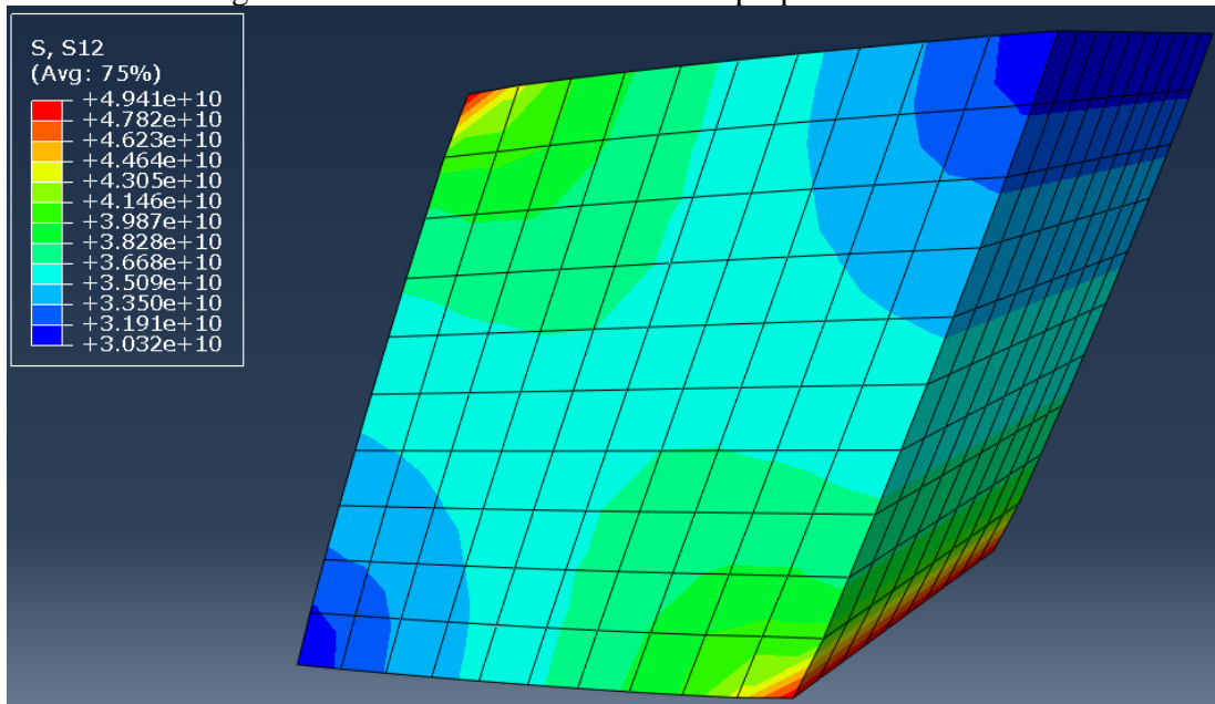
Figure 19. The shear stress field of the ABAQUS.
