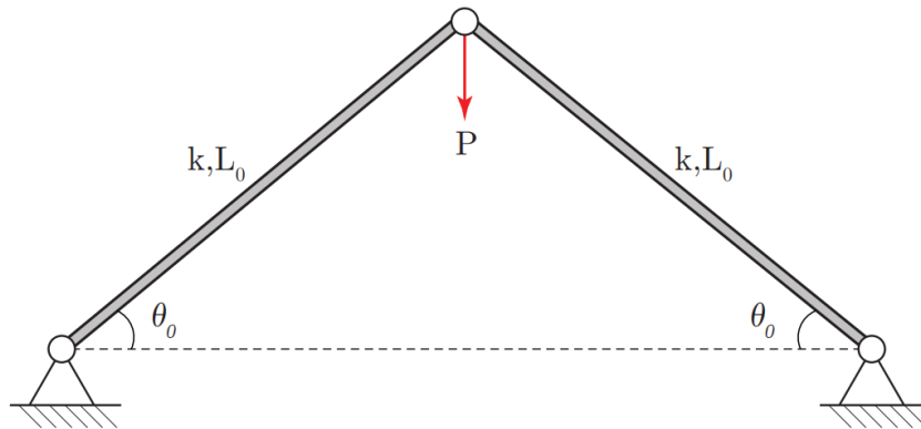
Figure 6. The configuration of the geometric nonlinearity problem.
