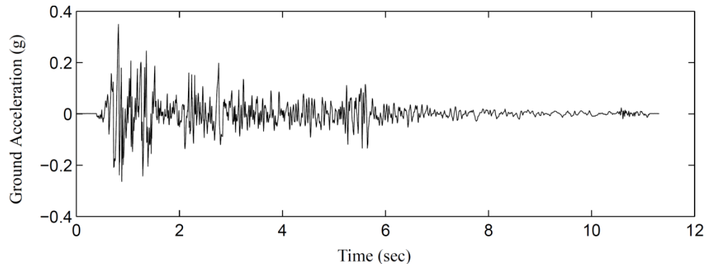
Figure 5. Time scaled NS component of the ground acceleration for the 1940 El Centro earthquake [4]
