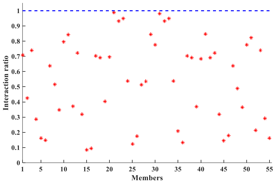
Figure 13. Members strength interaction ratio of 5×5 frame with fully moment connections
